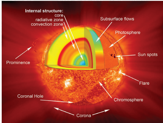
An illustration of the sun's internal core.
