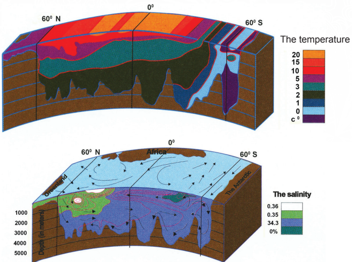
Vertical illustrative picture of the ocean showing the diversity in physical characteristics of the water mass. even on a vertical level.
