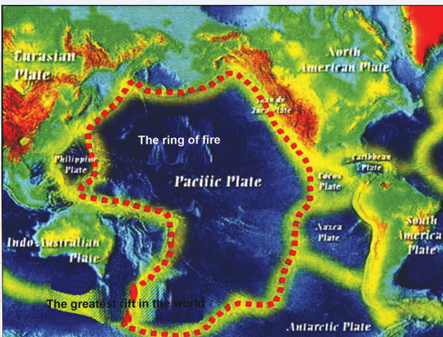
The Largest rifts on earth. covering 40.000 km
